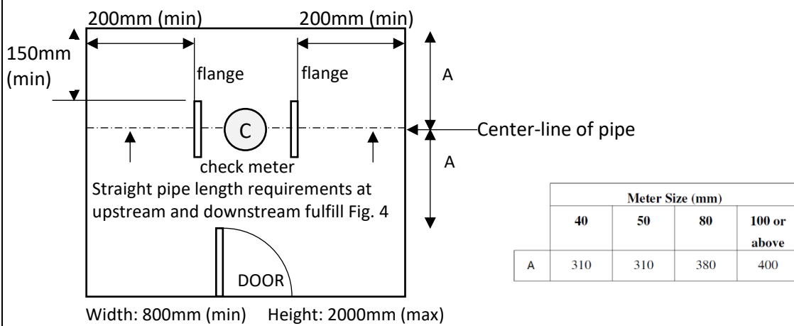
Fig. 8 Typical plan view of check meter position
