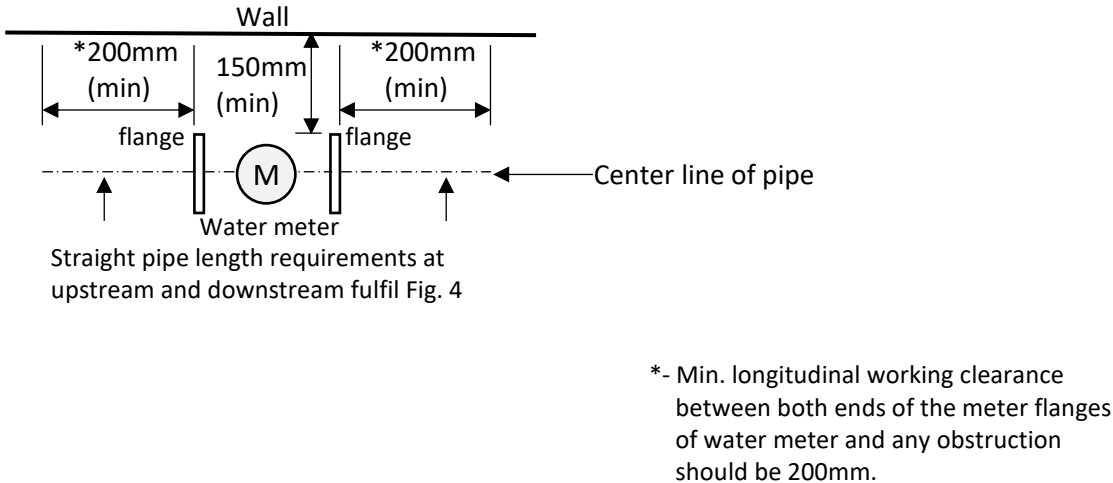
Fig. 8 Typical plan view of water meter position
