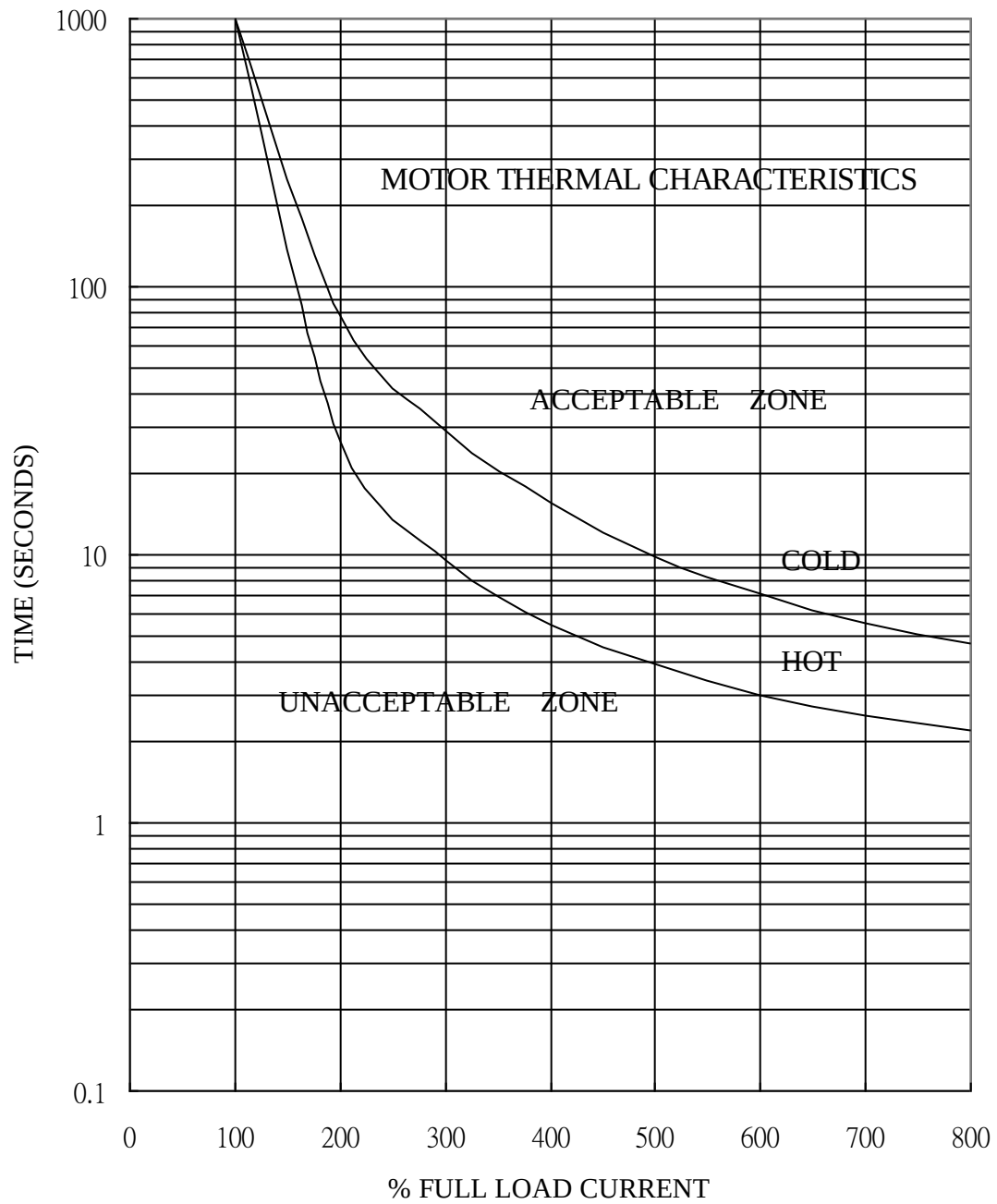
Motor Short-time Overload Withstand Characteristics
