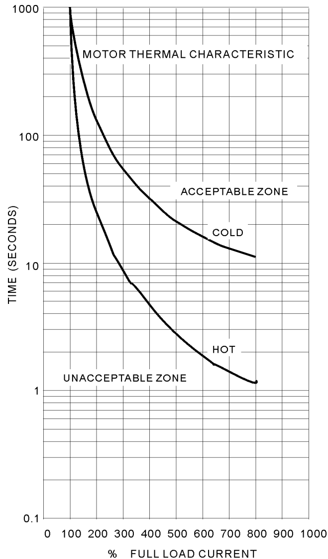
Motor Short-time Overload Withstand Characteristic
