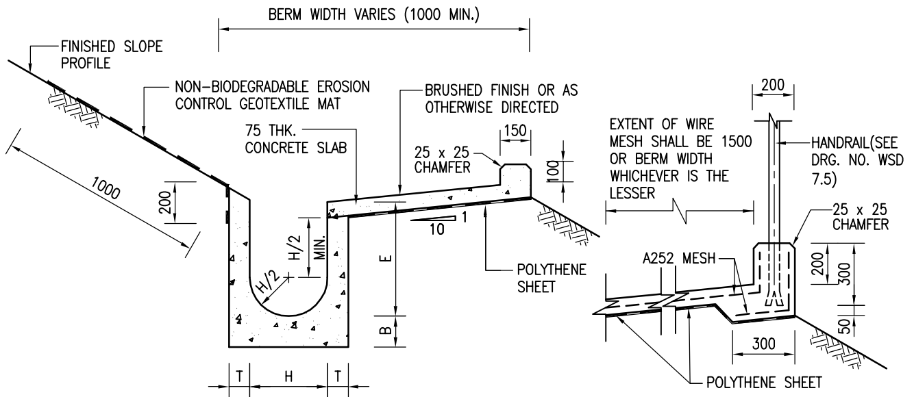
DETAILS OF BERM WITH HANDRAIL
