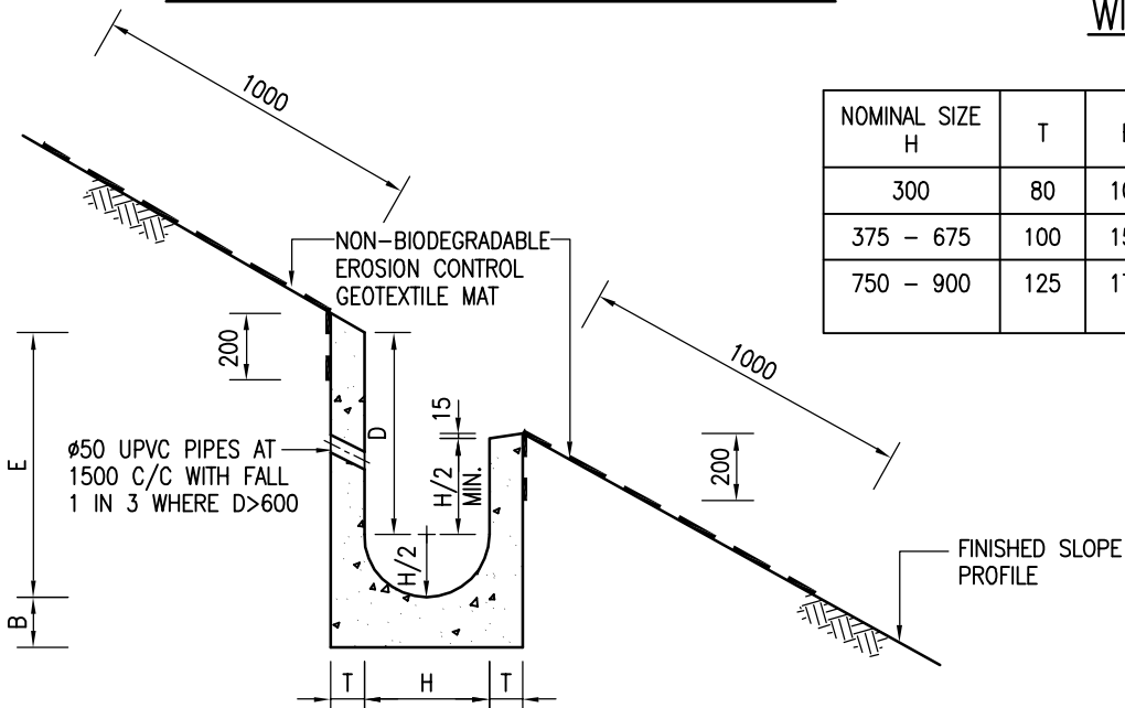
U-CHANNEL NOT CONSTRUCTED ON BERM
