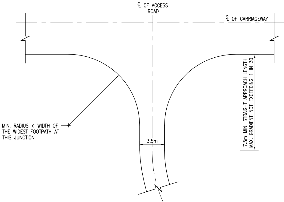
JUNCTION DETAIL
