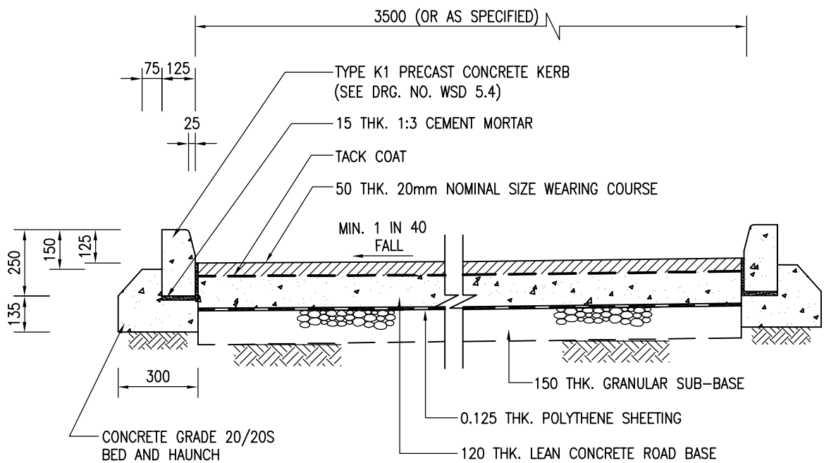
GENERAL DETAILS – FLEXIBLE CARRIAGEWAY
