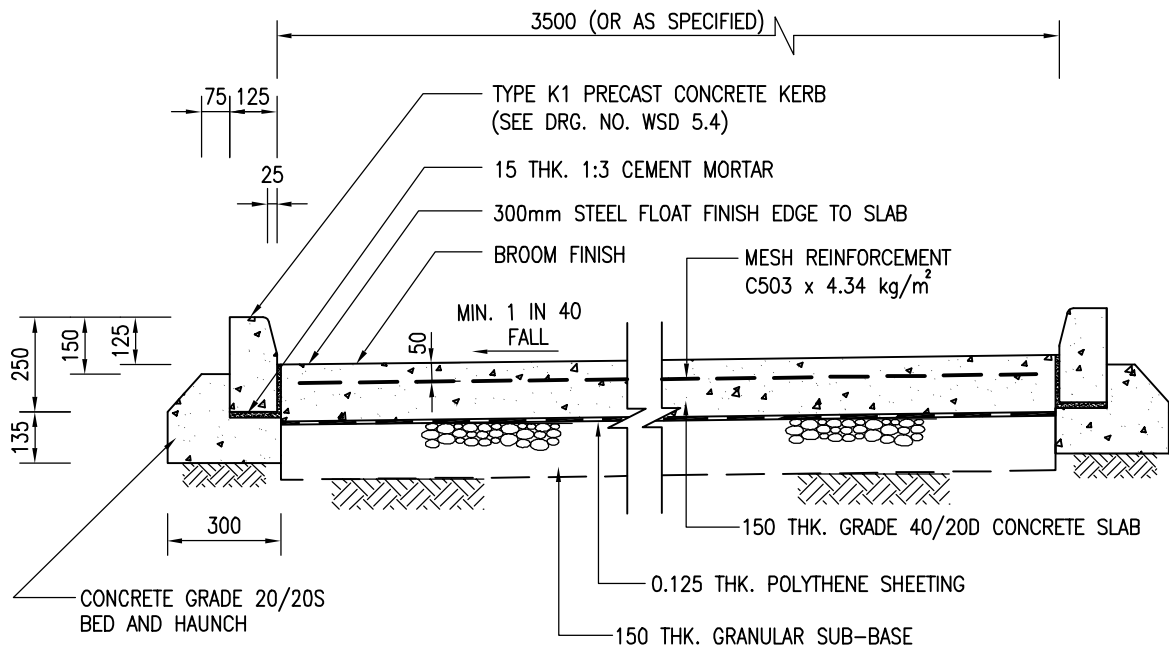
GENERAL DETAILS – CONCRETE CARRIAGEWAY
