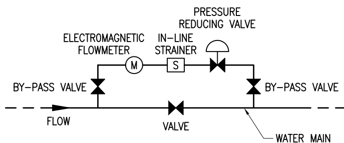
ARRANGEMENT OF FLOWMETER, IN-LINE STRAINER AND PRESSURE REDUCING VALVE
