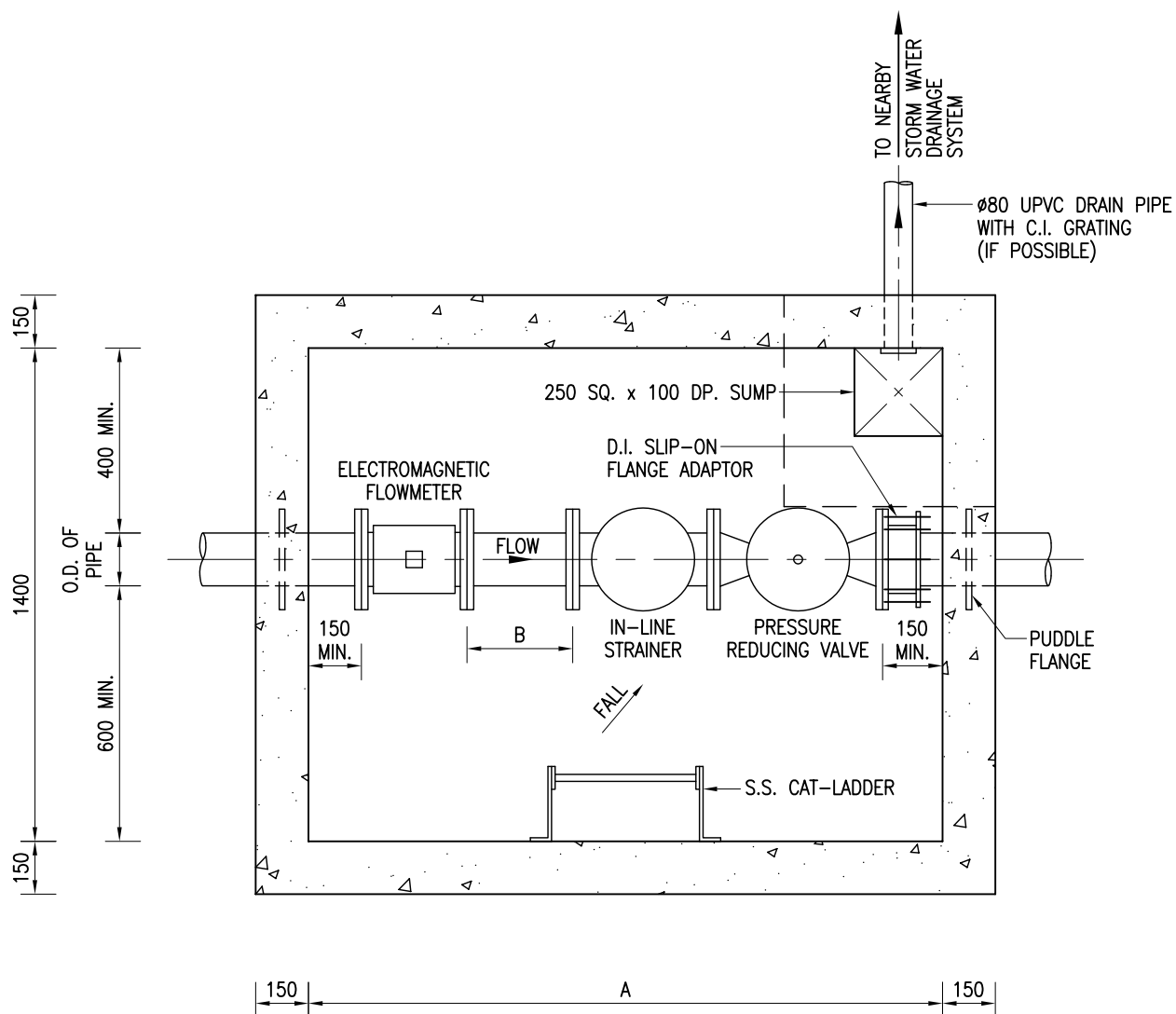
SECTIONAL PLAN
