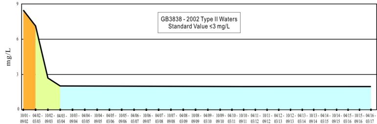
Nitrate
