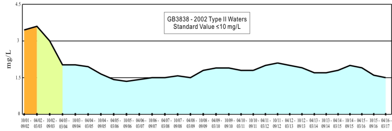
Nitrate
