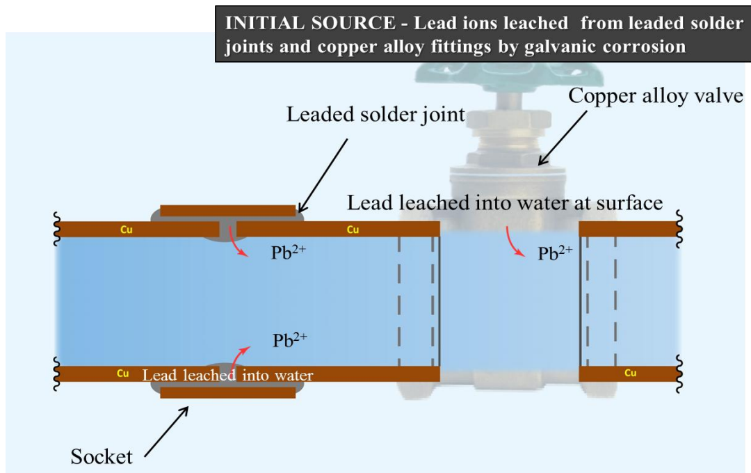
Figure 2.8(a) Leaching of lead from leaded solder joints and copper alloy fittings
